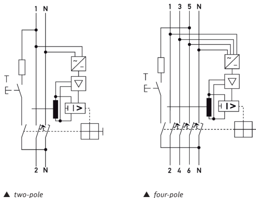
▲ two-pole
